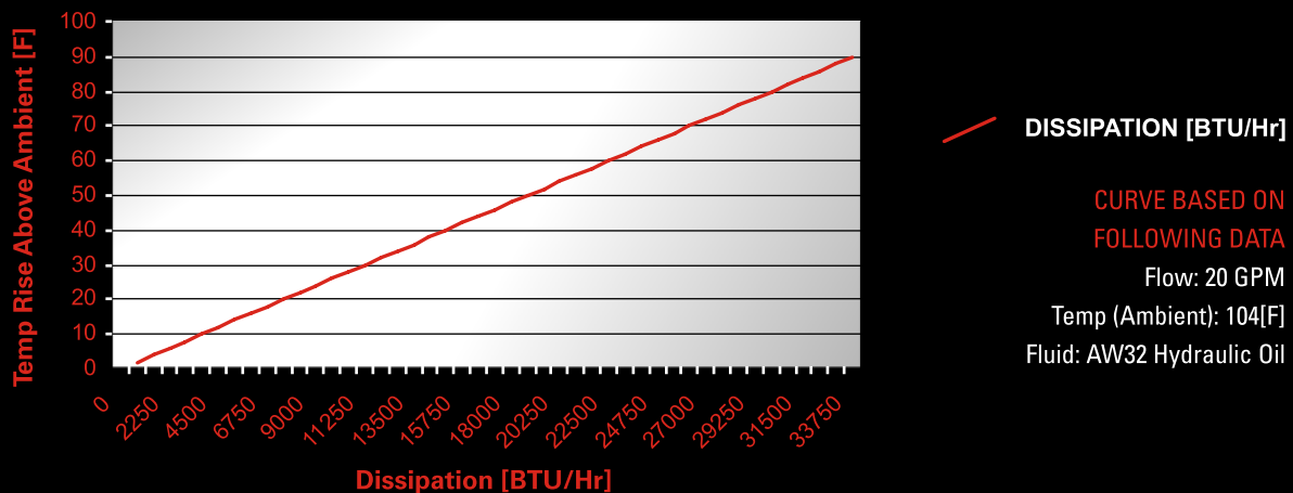
PERFORMANCE CURVE - THERMINATOR
